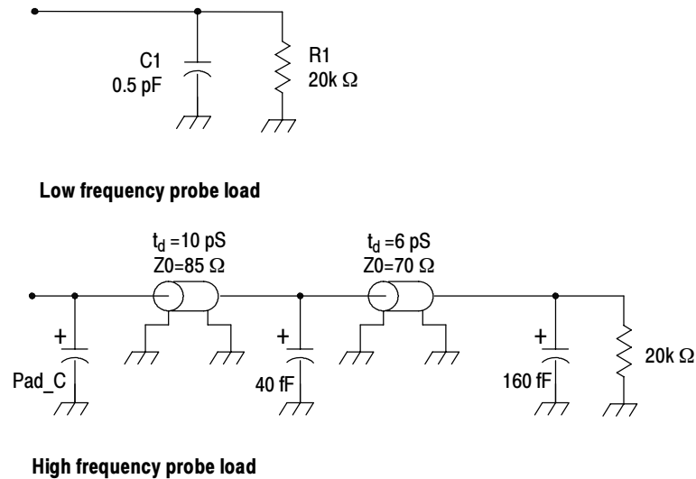
Figure 22: High-Density probe load model
