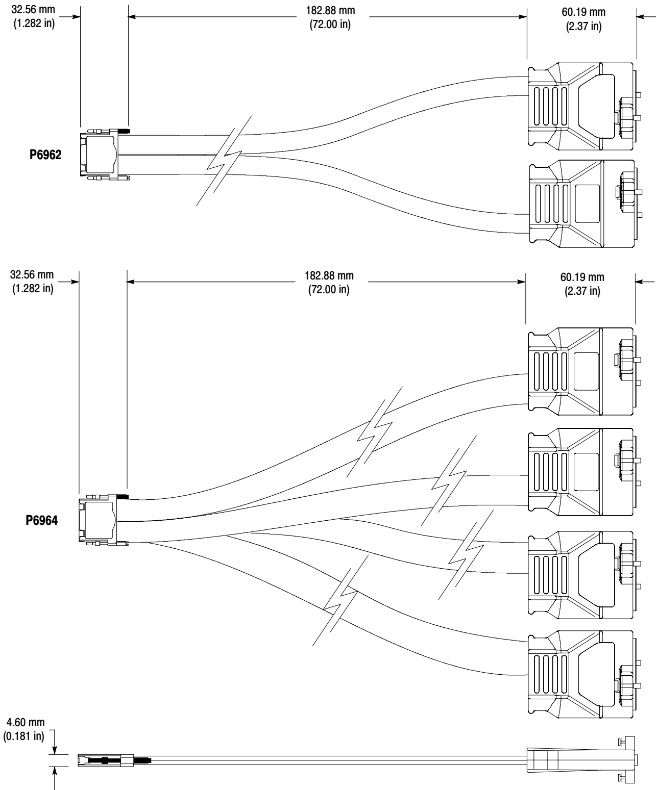
Figure 16: P6962 and P6964 probe dimensions
