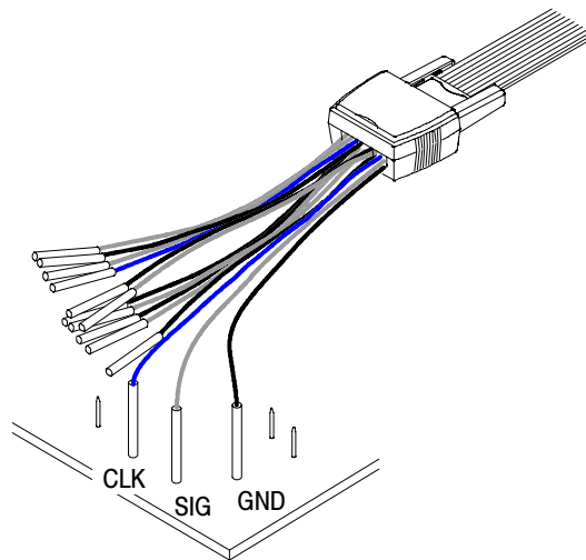
Figure 12: Using the flying lead set to connect to the target system
