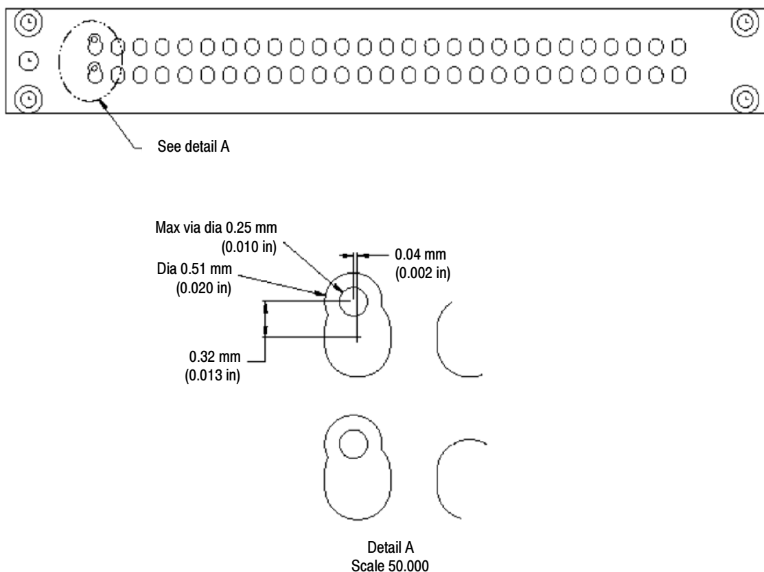
Figure 24: Optional Via-in-Pad placement recommendation
