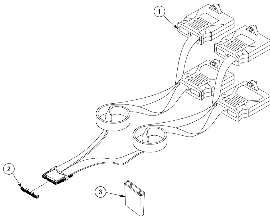
Figure 33: P6964 High-Density probe accessories
