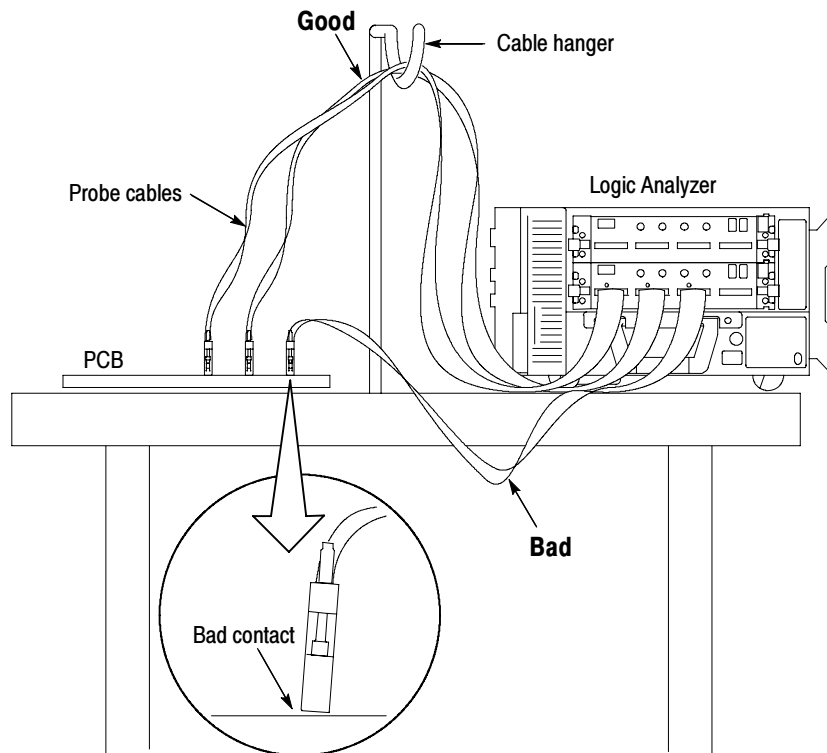
Figure 13: Proper dressing of the probe cables
