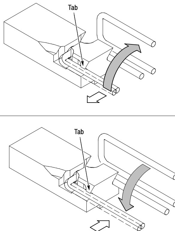
Figure 7: Replacing the wires on the retention posts
