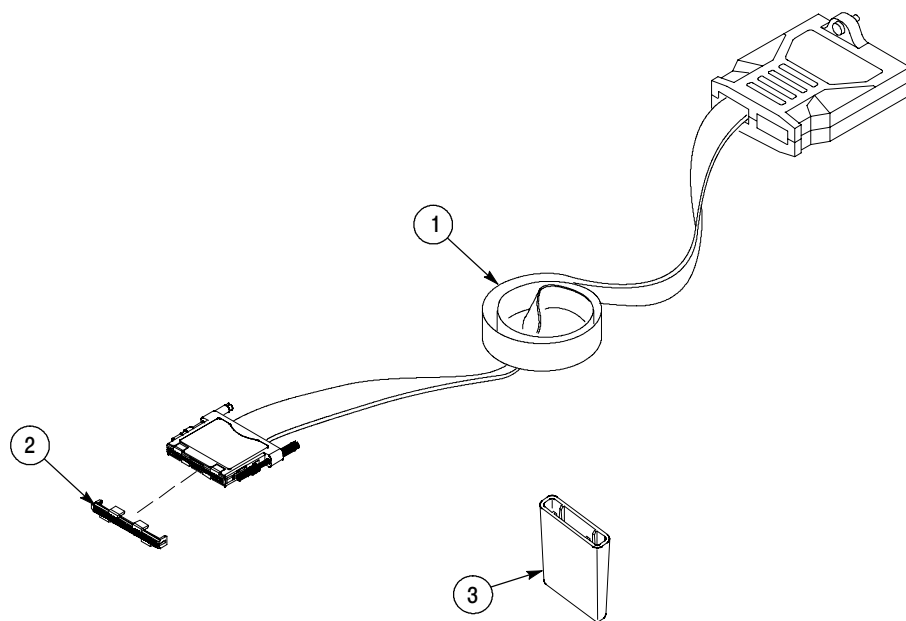
Figure 35: P6982 High-Density Differential probe accessories
