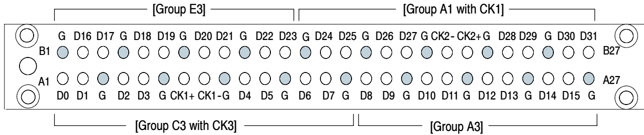
Figure 27: P6964 single-ended PCB footprint pinout detail
