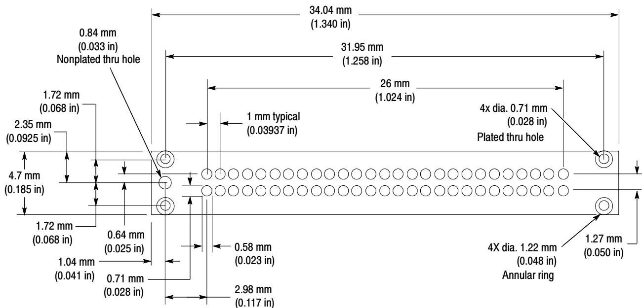
Figure 23: Probe footprint dimensions on the PCB
