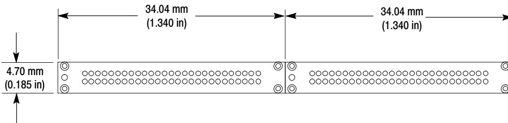
Figure 20: End-to-end layout
