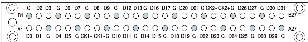
Figure 25: P6960 single-ended PCB footprint pinout detail
