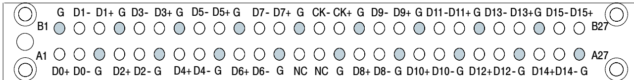
Figure 28: P6980 differential PCB footprint pinout detail
