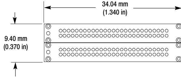
Figure 19: Side-by-side layout
