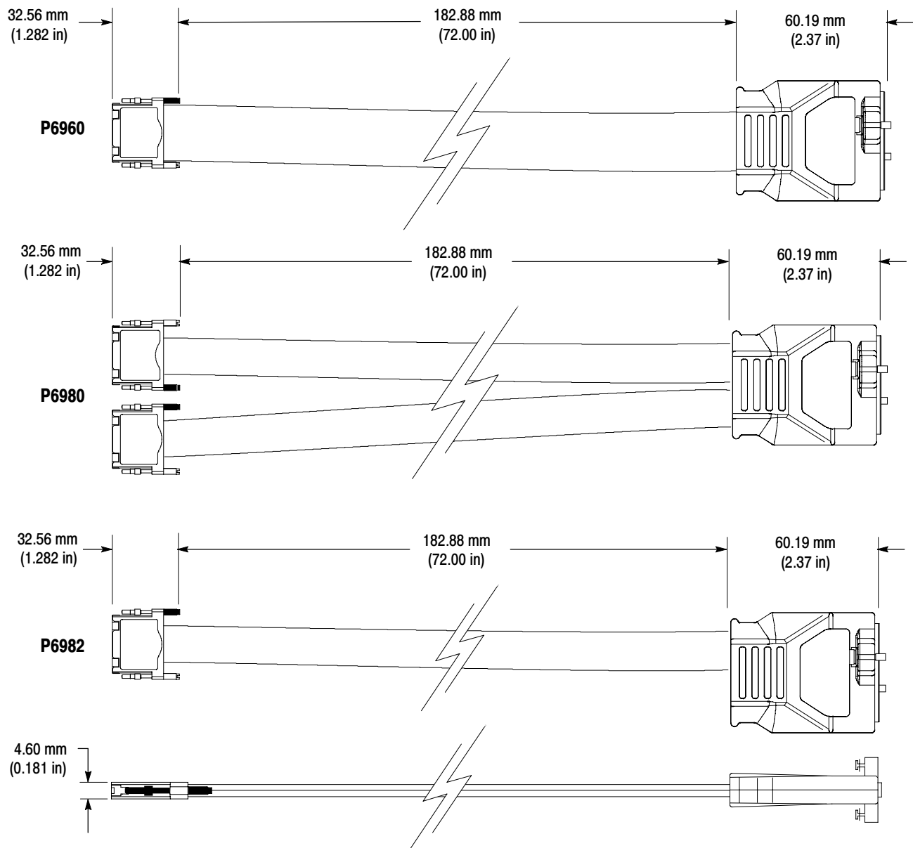
Figure 15: P6960, P6980, and P6982 probe dimensions
