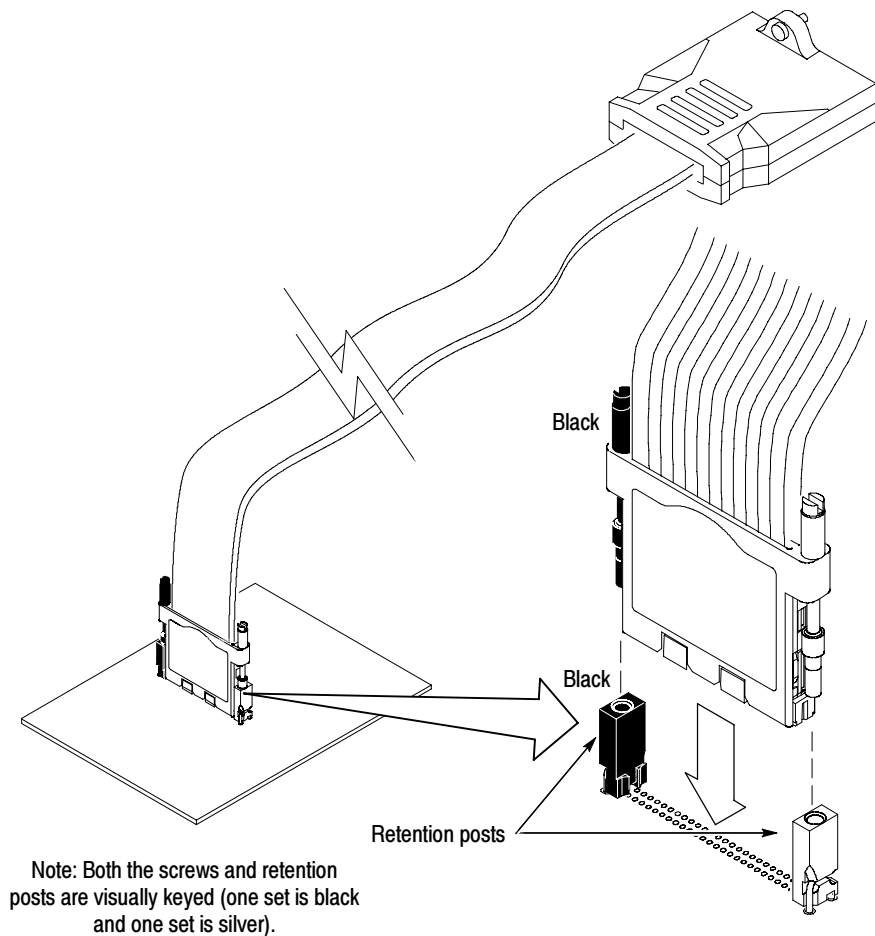
Figure 11: Connecting the probes to the target system
