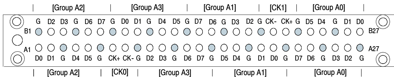
Figure 26: P6962 single-ended PCB footprint pinout detail
