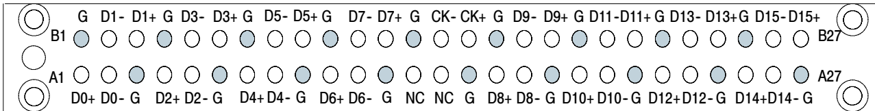
Figure 29: P6982 differential PCB footprint pinout detail
