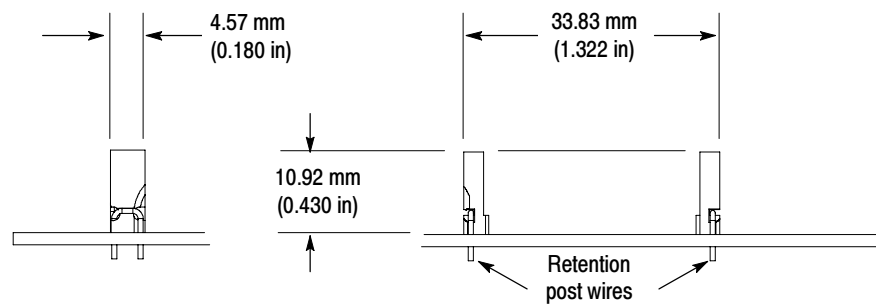
Figure 17: Retention post dimensions
